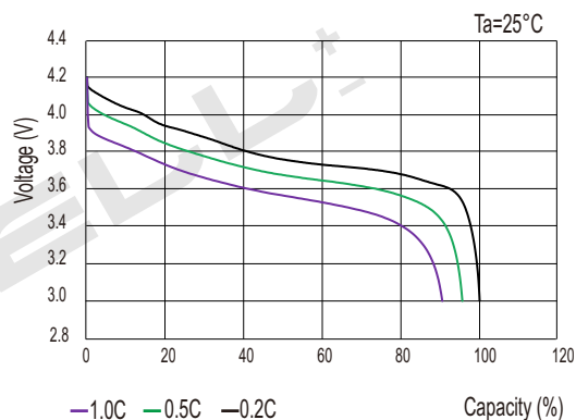
Discharge Characteristics (by rate)
