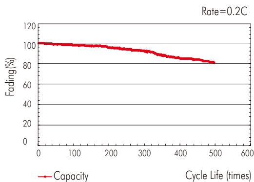
Cycle Life ( 23 \pm 2^\circ\text{C} )
