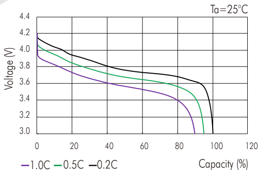
Discharge Characteristics (by rate)
