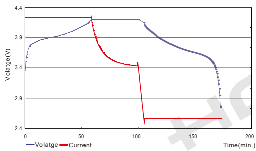
Charge & Discharge (25°C)
