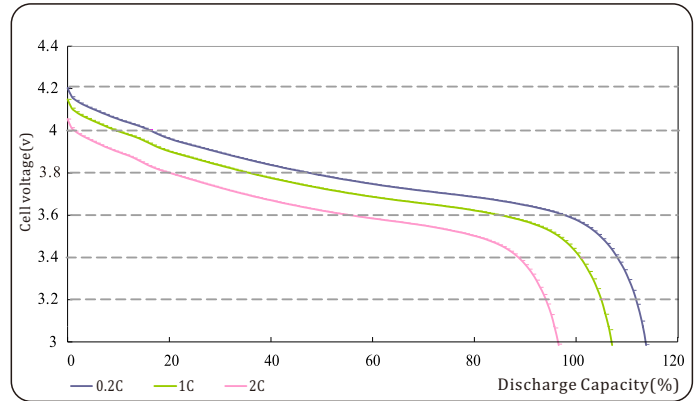
Discharge Characteristics (Rate)
