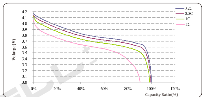
Discharge Characteristics (Rate)
