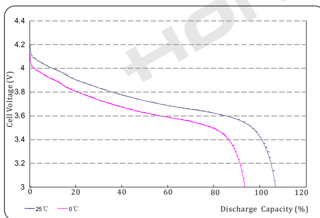
Discharge Characteristics in Different Temperature
