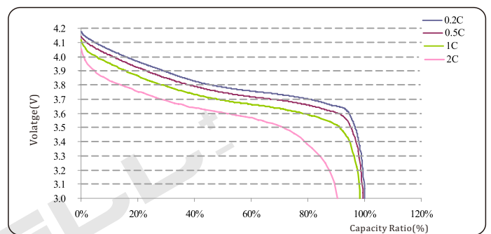
Discharge Characteristics (Rate)
